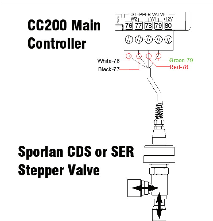
Main Controller Stepper Valve Wiring
