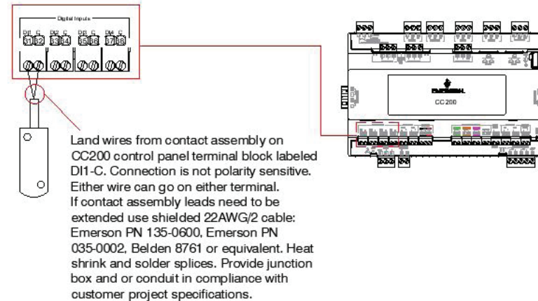
118-4101 Door Switch Mounting for Hinged Doors
