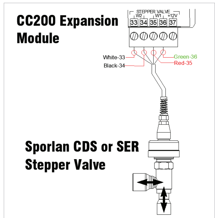
Expansion Module Stepper Valve Wiring
