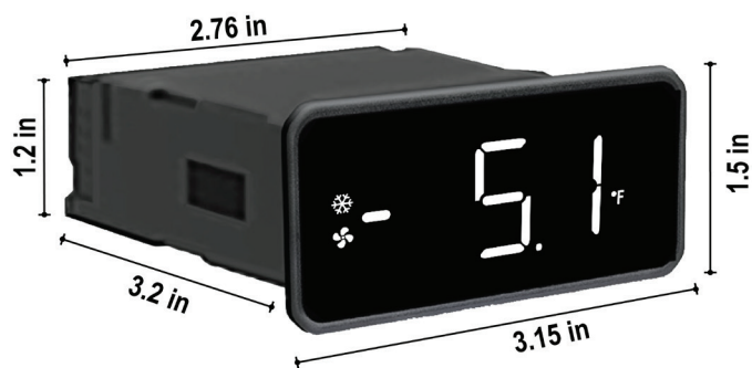
CC200 Case Display Dimensions
